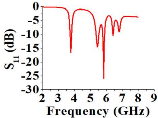
Fig. 15: S_{11} parameter of conventional antenna Fig. 16: S_{11} parameter of proposed antenna
