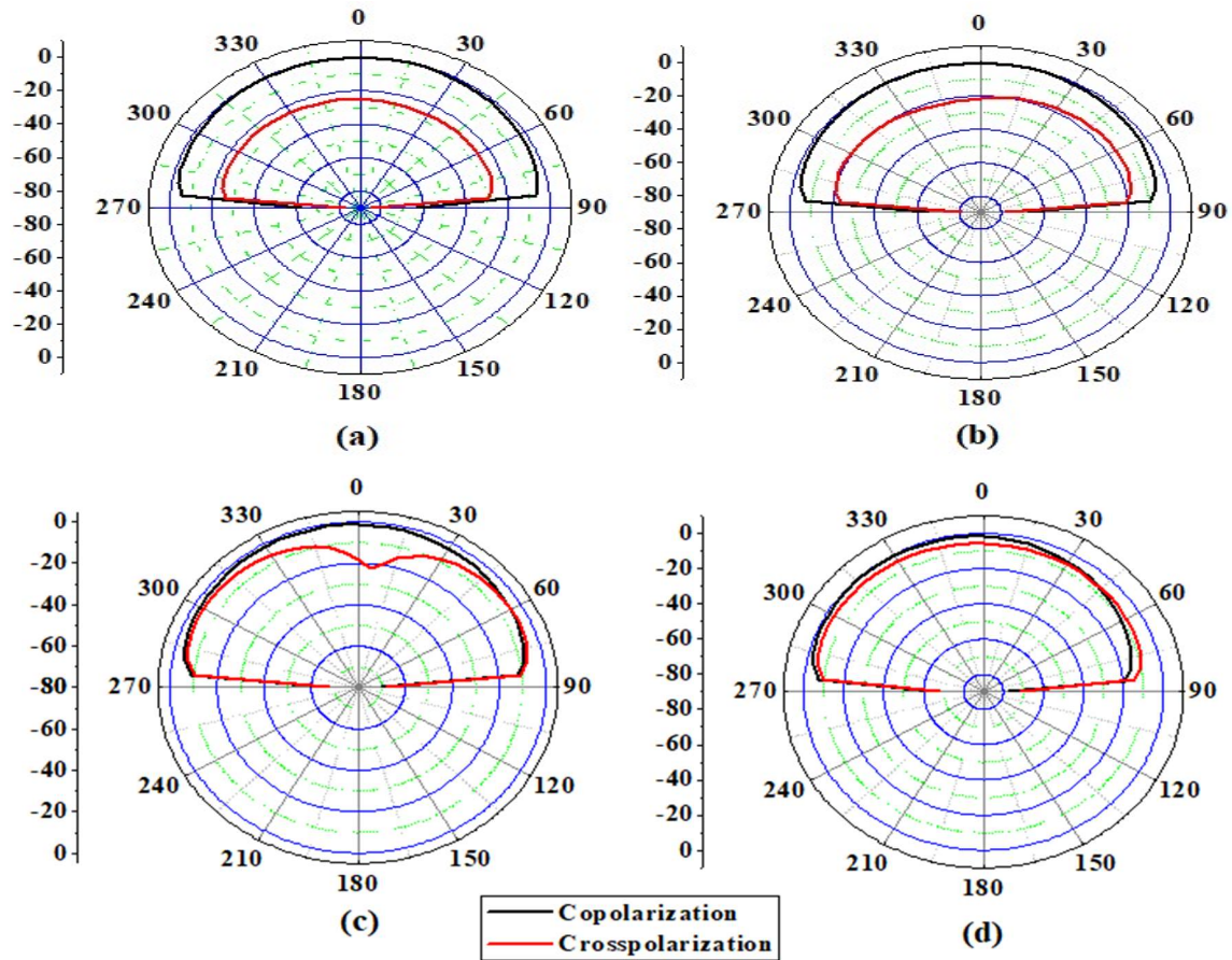
Figure 19: Normalized E-plane radiation pattern of the proposed antenna at (a) 3.79 GHz, (b) 5.44 GHz, (c) 5.84 GHz and (d) 6.44 GHz
