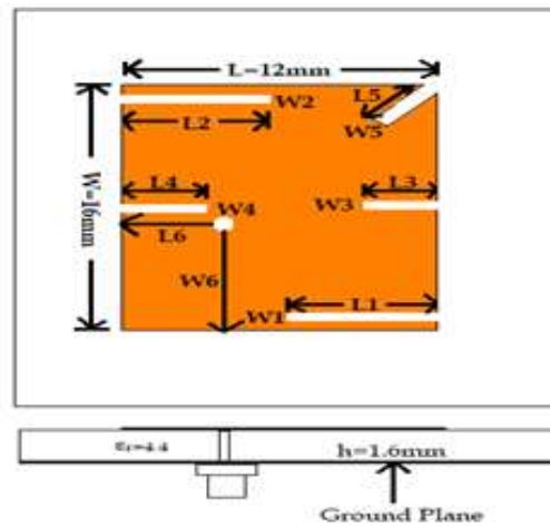
Figure 2: configuration of Antenna 2 (Proposed Antenna)
