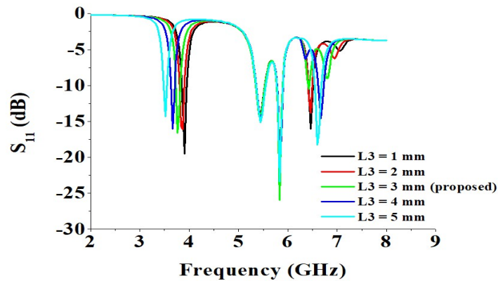
Figure 8: Variations of S_{11} for different values of L_3 parameter
