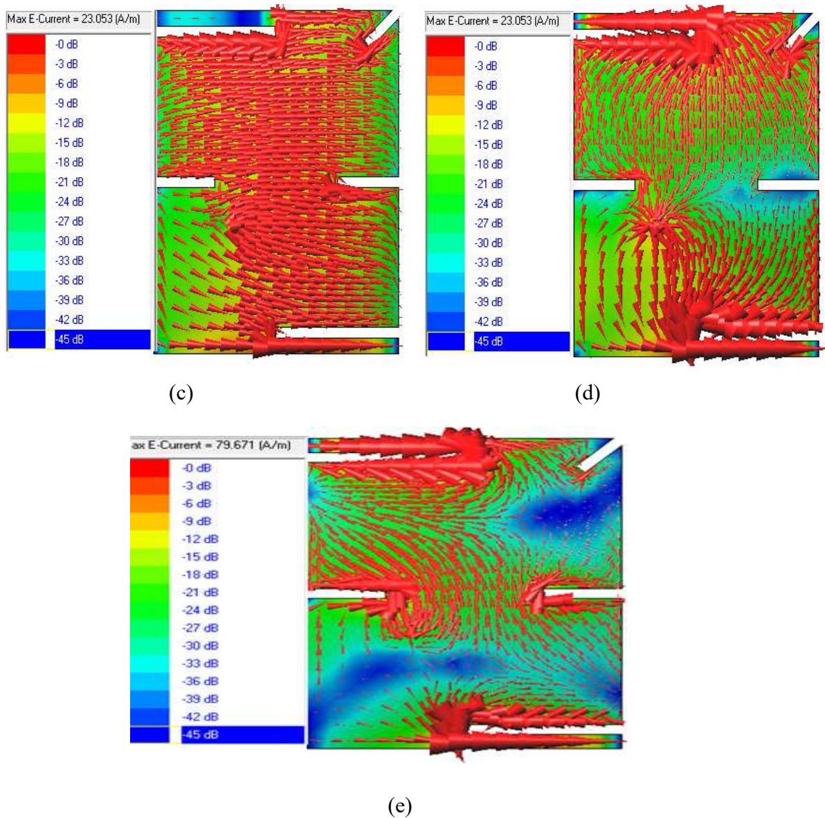
Figure 14: Surface current distribution for Conventional antenna at (a) 5.5 GHz and for the proposed antenna at (b) 3.79 GHz, (c) 5.44 GHz, (d) 5.84 GHz and (e) 6.44GHz
