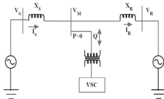
Figure-1 STATCOM model
