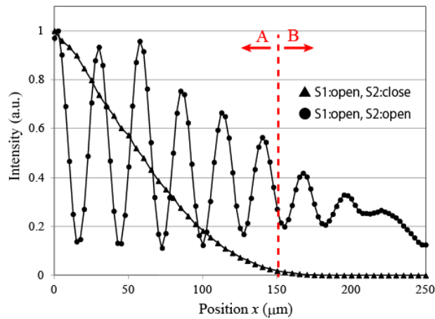
Fig. 3 Intensity distribution of light passing through a single slit and double-slit. The intensity was observed with a CCD placed at the end of the optical fiber. In the case of a single slit, diffracted waves were hardly observed where x was 150 \mu\text{m} or greater (region B), but when both slits were opened, interference fringes were observed.
