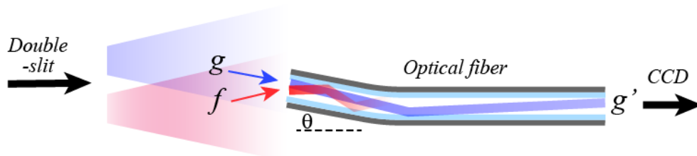
Fig. 4 Schematic diagram of the incident angle and propagation of light in the optical fiber. The light waves f and g emitted from the respective slits are superposed and enter the fiber, but f does not match the mode of the optical fiber, so it decays rapidly in the optical fiber. Although the light wave detected by the CCD is g' , the interference effect is observed.
