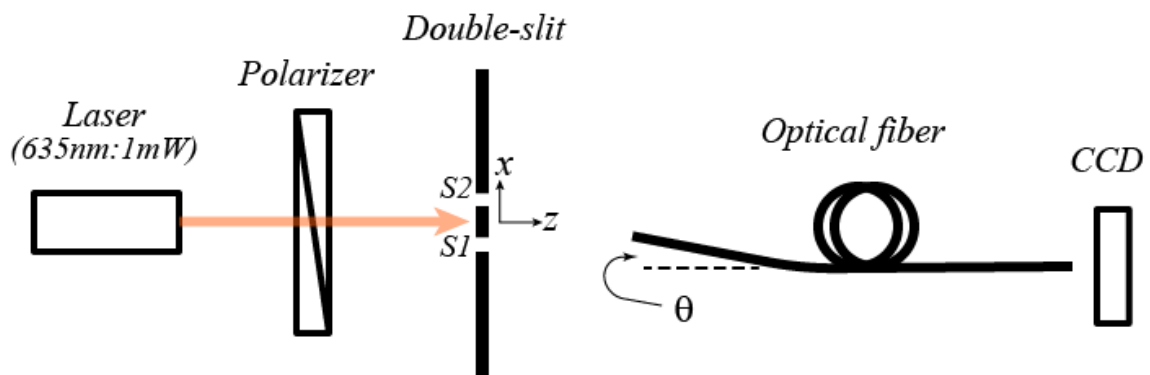
Fig. 1 Apparatus to observe interference fringes using an optical fiber. The laser beam passes through a polarizing plate (45 degrees) and a double-slit to form interference fringes. The interfering light enters an optical fiber (inclination \theta ) and is measured by a CCD placed at the end. The optical fiber is scanned in the x and z directions by motorized stages to obtain an intensity distribution.
