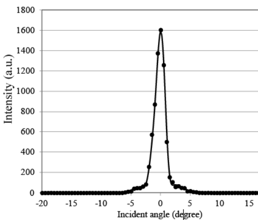
Fig. 2 Correlation of the incident angle and transmitted light of a single-mode optical fiber.
