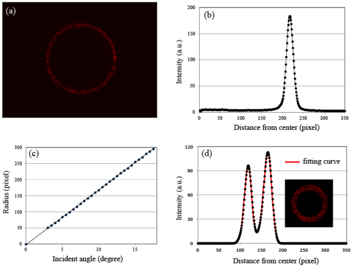
Fig. 5 Observation of photon movement using an MMF. (a) Image of a circle at the exit surface of the fiber when light entered the fiber obliquely, (b) the intensity distribution with respect to the distance from the center of the circle, (c) the correlation between the incident angle and the radius of the circle, and (d) the intensity distribution when light waves entered from two directions.
