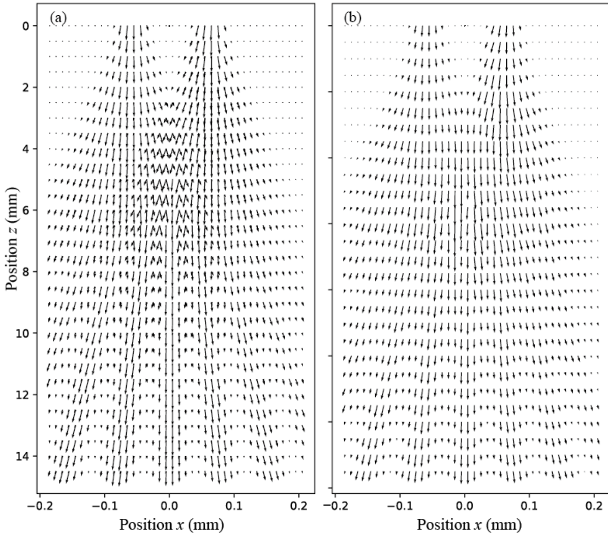
Fig. 6 Vector diagram showing the photon movement near the double-slit (a) and the averaged diagram (b).
